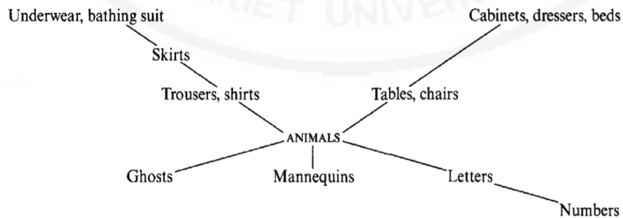
DIAGRAM 12.1. Structure of the tua category in Thai
